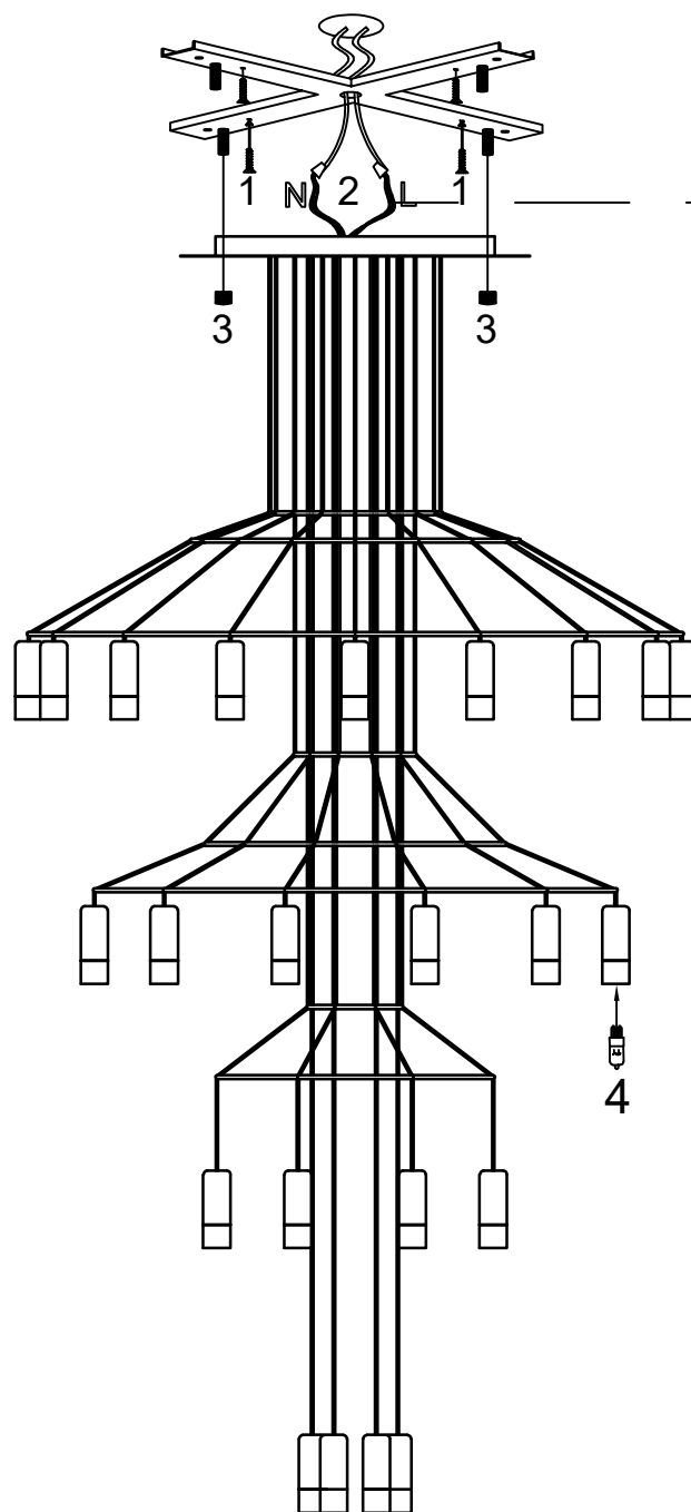
Wiring instructions
