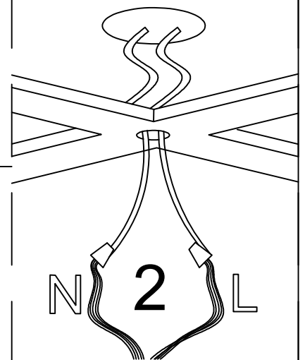
Wiring instructions
