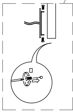
3 Connect the lamp body to the hanging plate
