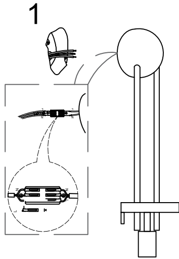
The wires in the home are connected to the wires in the lamps through the wire terminals
