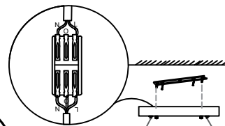
Install the hanging plate on the ceiling
