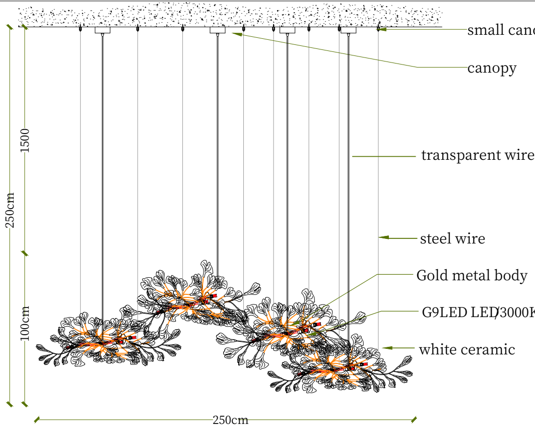
main view
