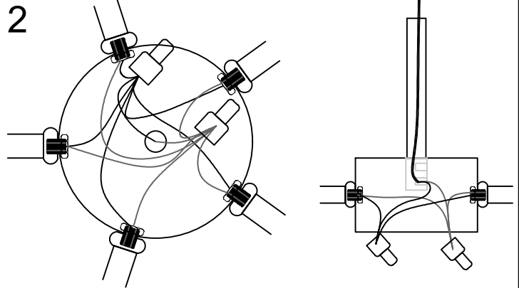
2 The lines of the same color are connected together and then connected with two lines that are respectively connected with the main line
