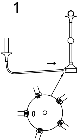
1 The lamp arm is connected to the center post by screws
