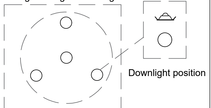
Ceiling downlight hole diagram
