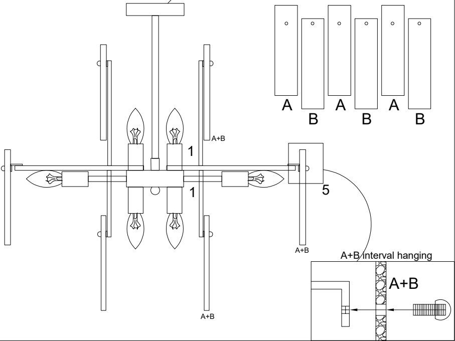
Enlarged Detail
