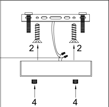
Enlarged Detail
