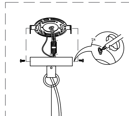
The side screws fix the lamp body to the ceiling plate
