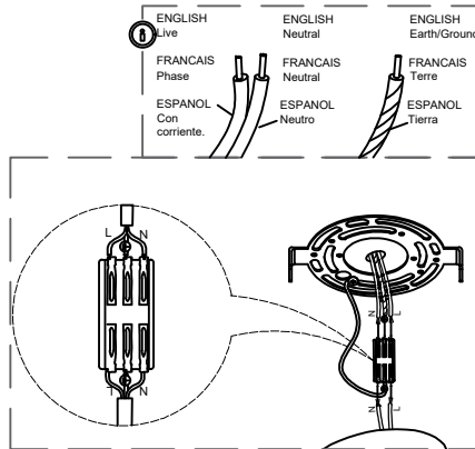
The wires in the home are connected to the wires in the lamps through the wire terminals
