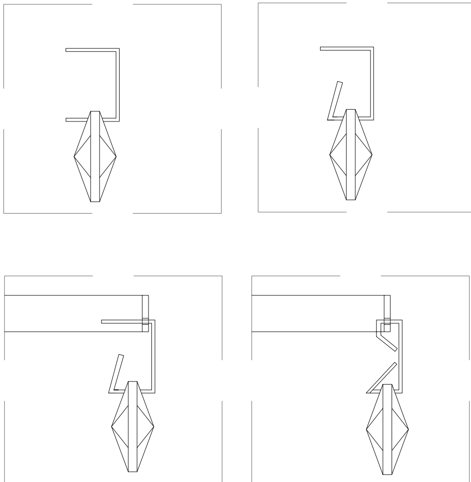
How to install crystal pendant
