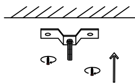
Install the hanging plate on the ceiling
