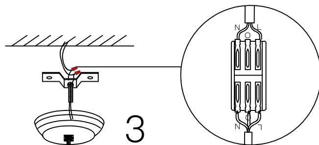
The electric wires in the home connect to the light fixtures
