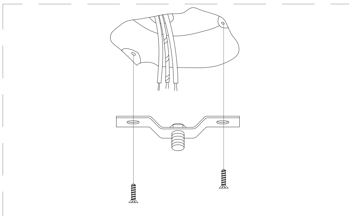
Fixed mounting plate
