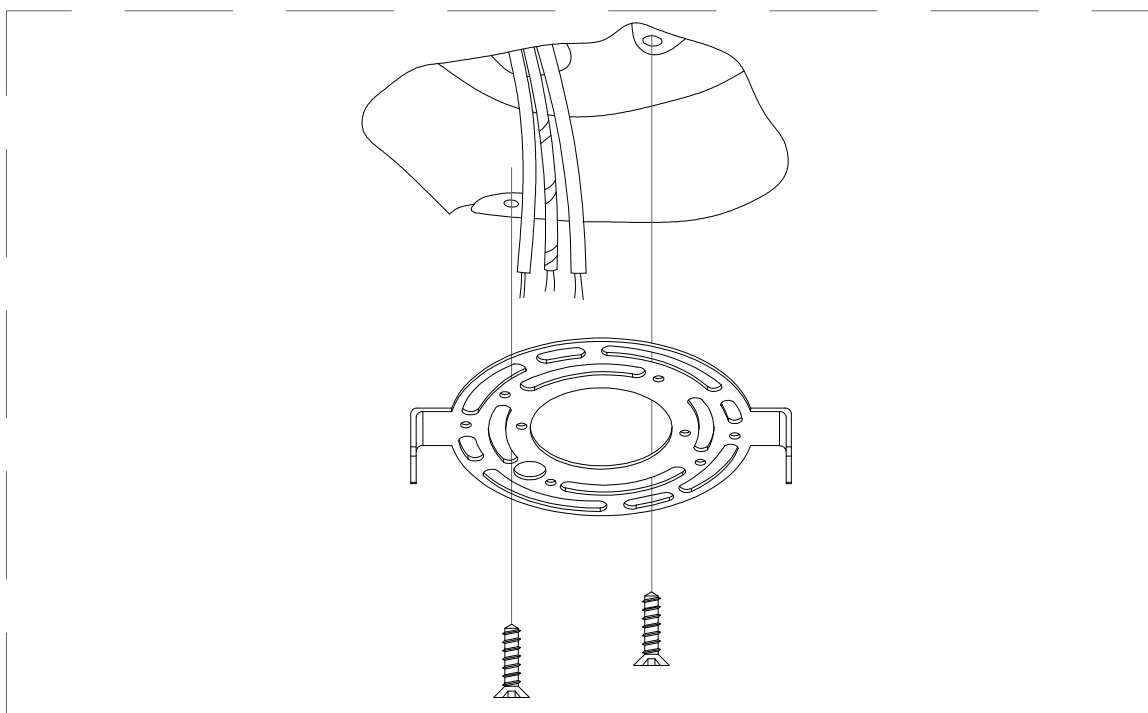
⑧: Fixed mounting plate
