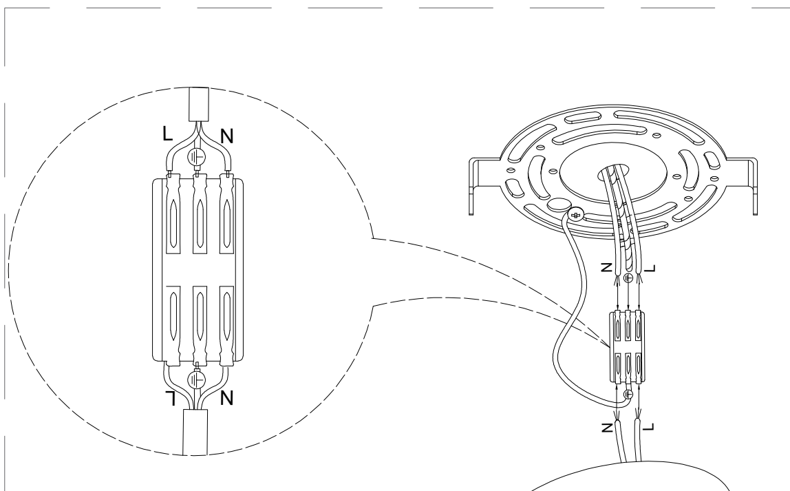
⑨: Connecting to pre-installed wiring in the ceiling
