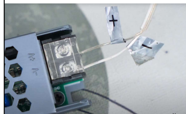
Transformer wiring method
