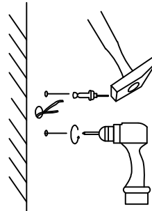
Drill holes in the wall and insert expansion screws
