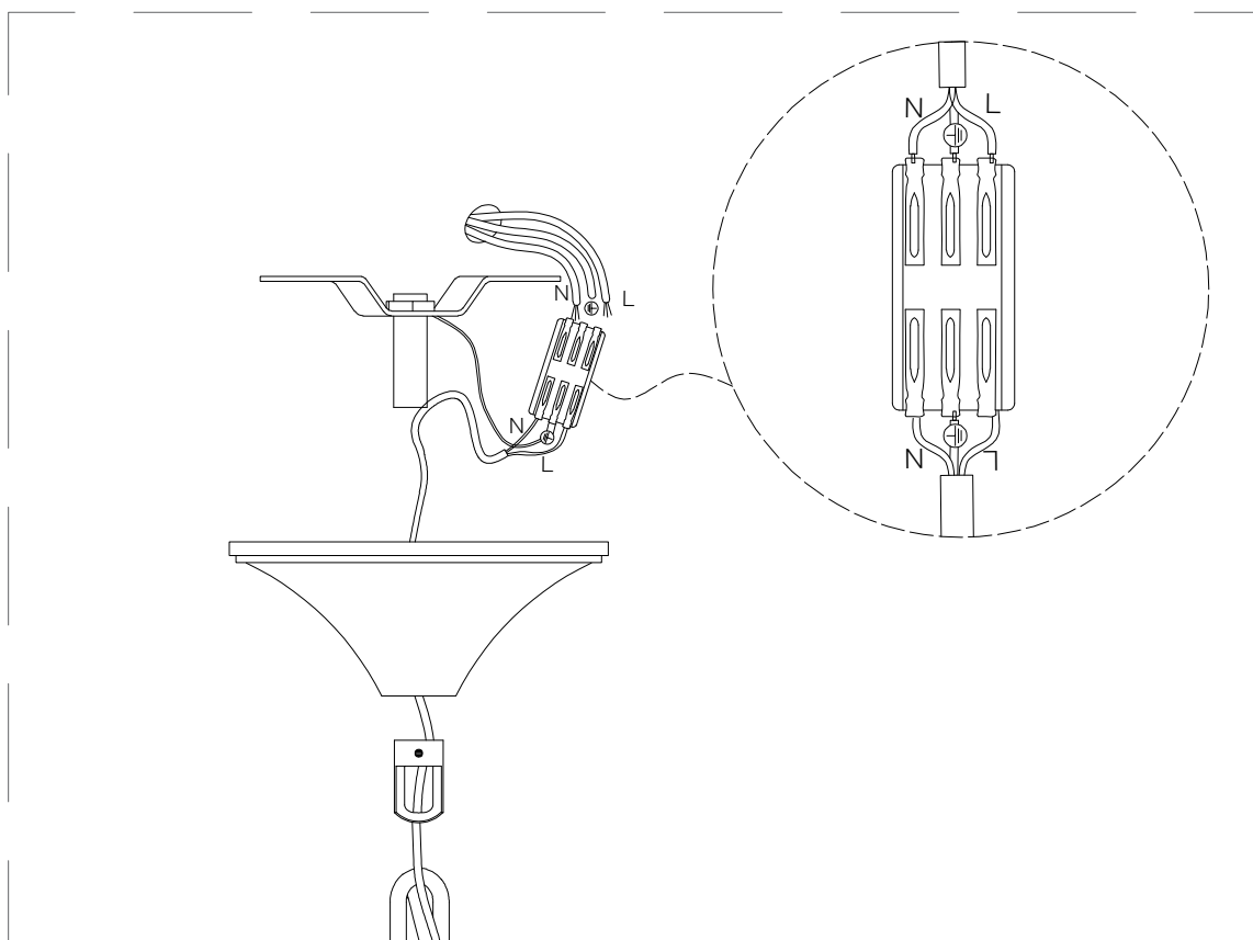
⑤: Connect the wires reserved in the ceiling.
