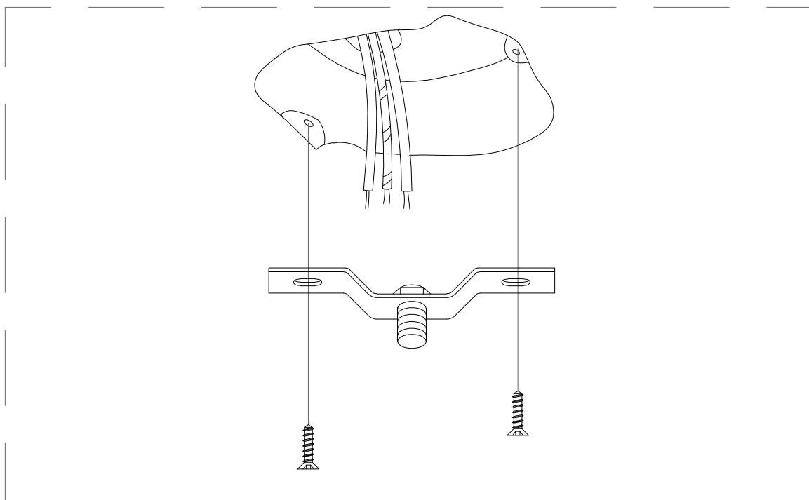
④: Fixed mounting plate
