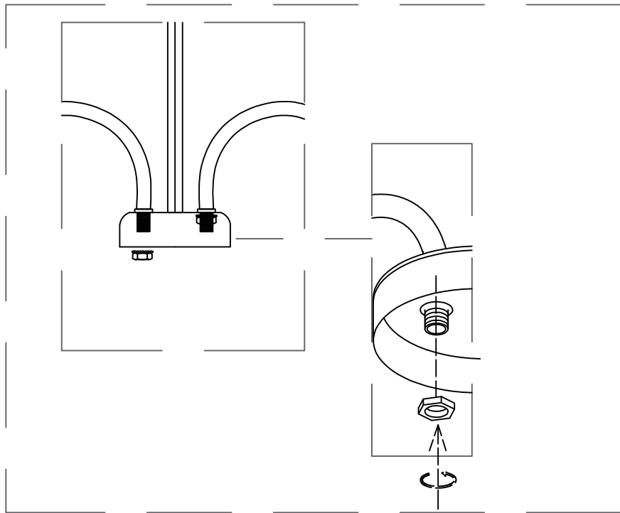
Assemble the Lamp Body
