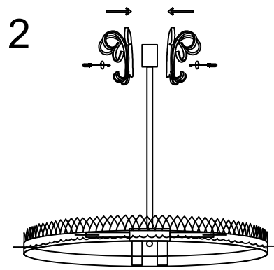
Mounting lamp body2
