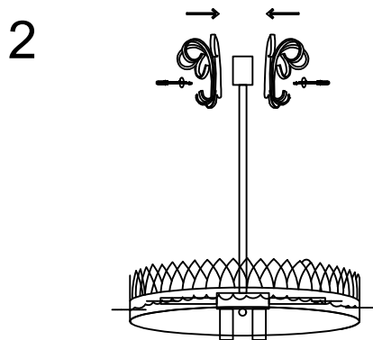
Mounting lamp body2
