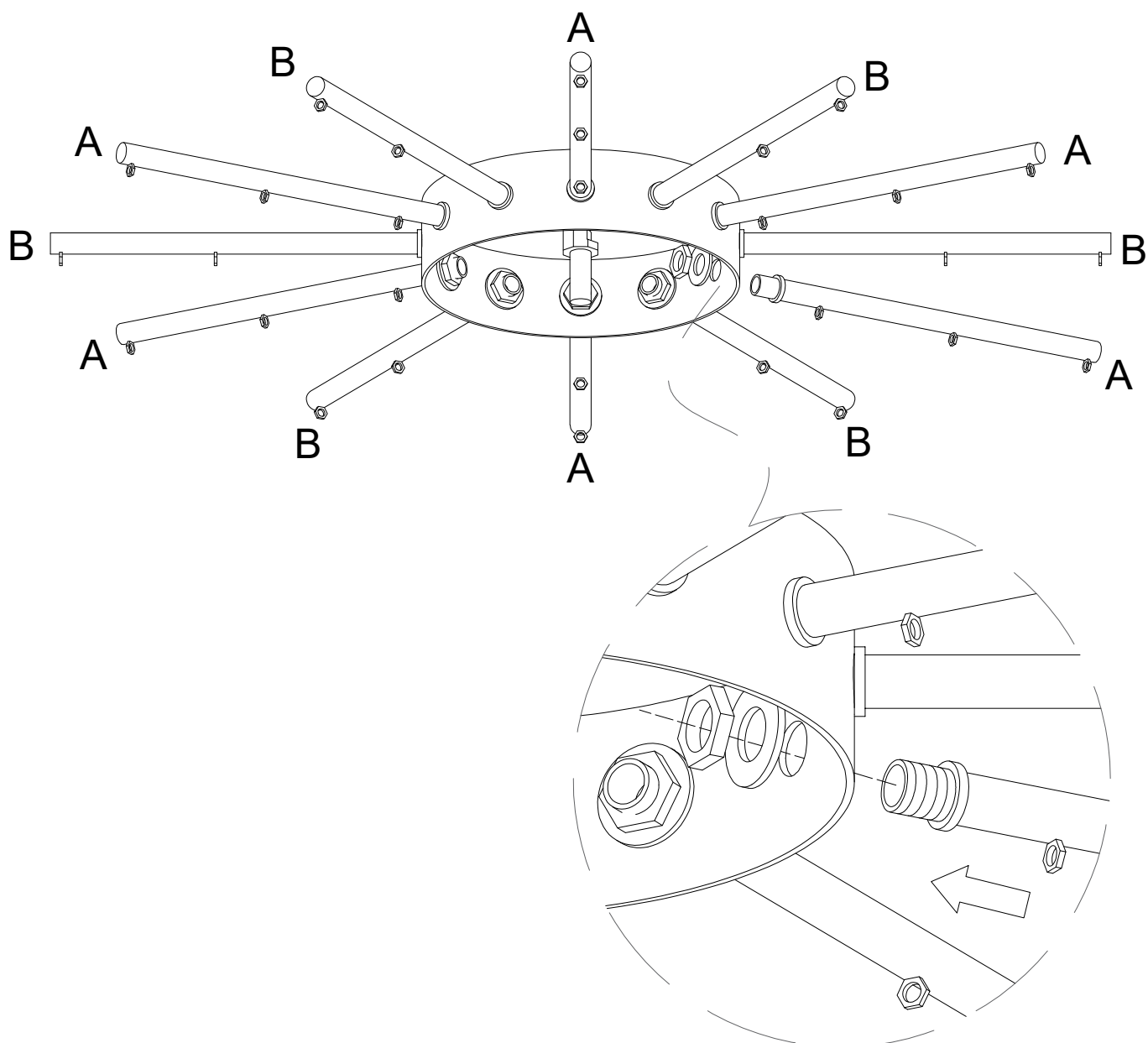
A/B Lamp Arms Installed at Intervals
