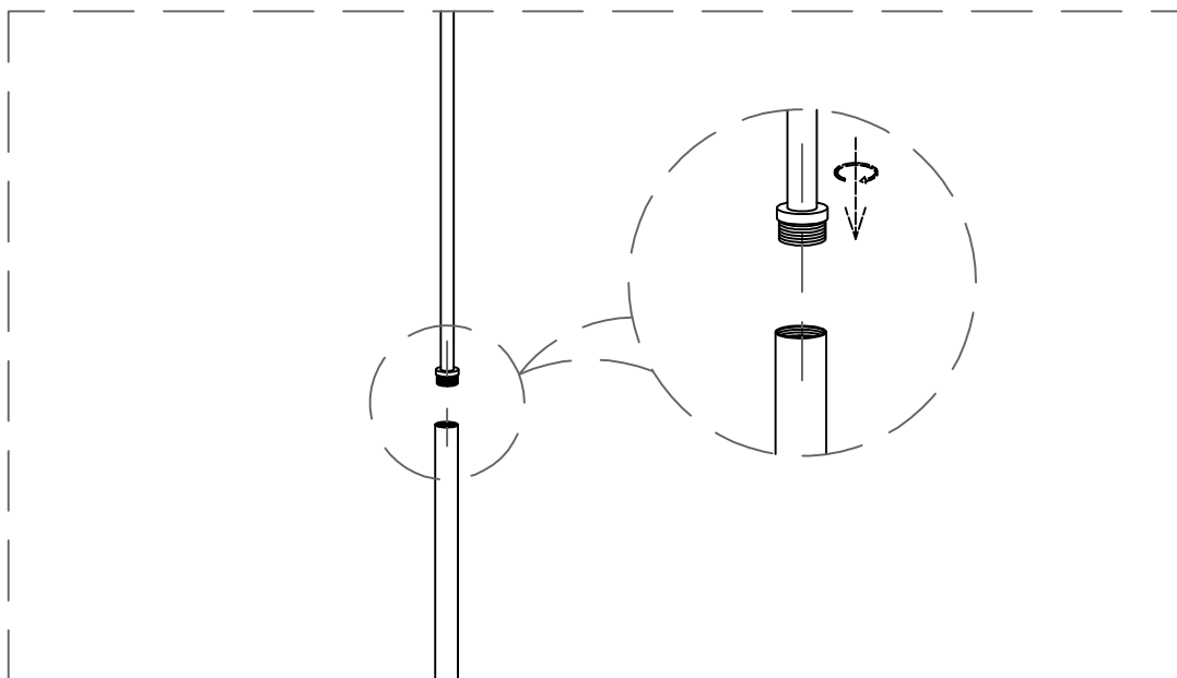
Connecting the middle rod
